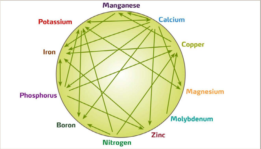
Mulders chart
